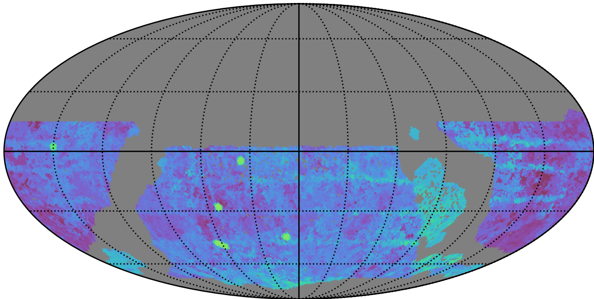
no_magell_roll_v3.4_10yrs WFD g band: Median Season Length
