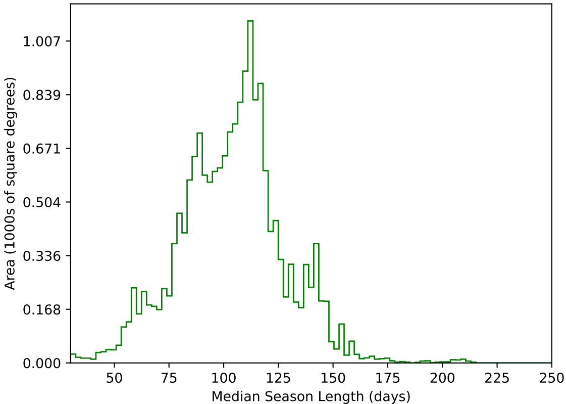
no_magell_roll_v3.4_10yrs WFD g band: Median Season Length
