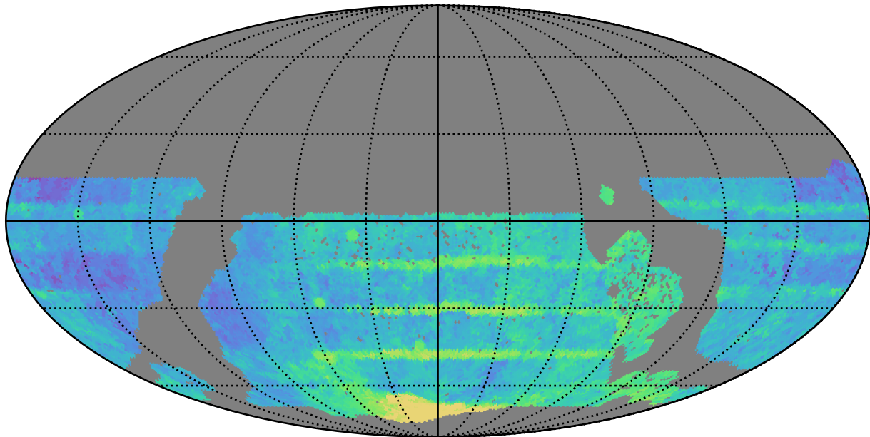
no_magell_roll_v3.4_10yrs WFD all bands: Median Season Length
