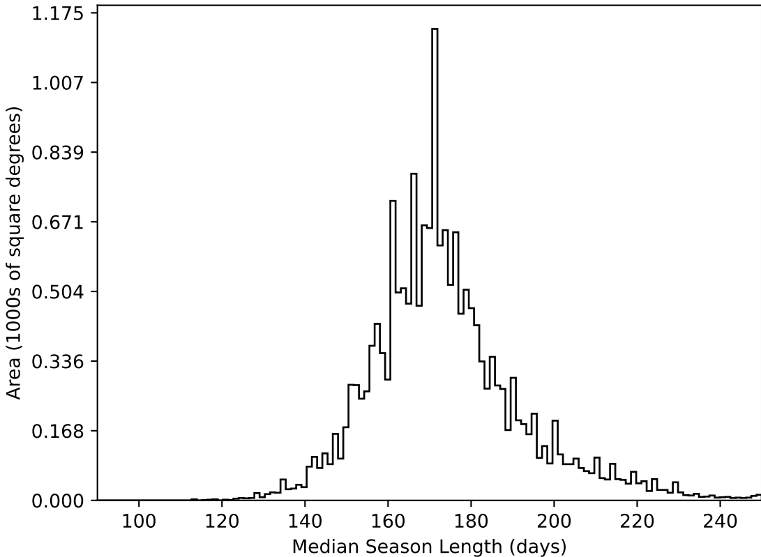
no_magell_roll_v3.4_10yrs WFD all bands: Median Season Length
