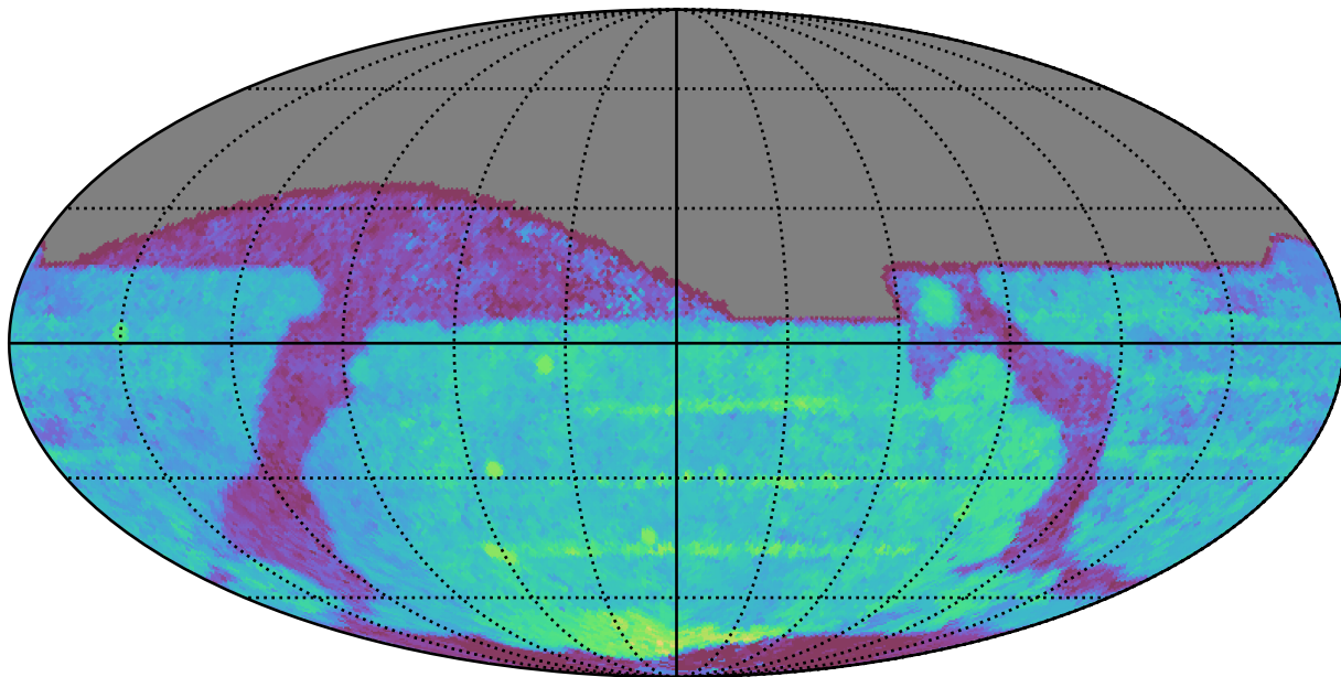
no_magell_roll_v3.4_10yrs All sky z band: Median Season Length
