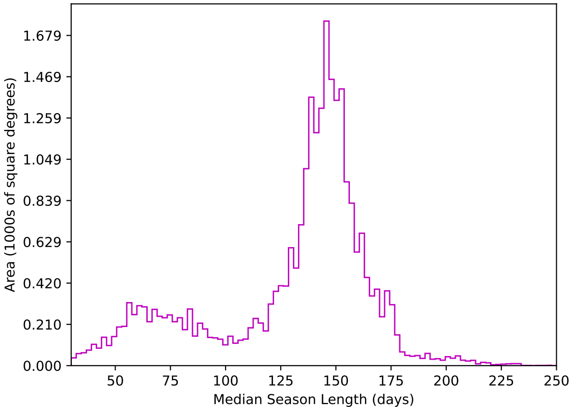
no_magell_roll_v3.4_10yrs All sky z band: Median Season Length
