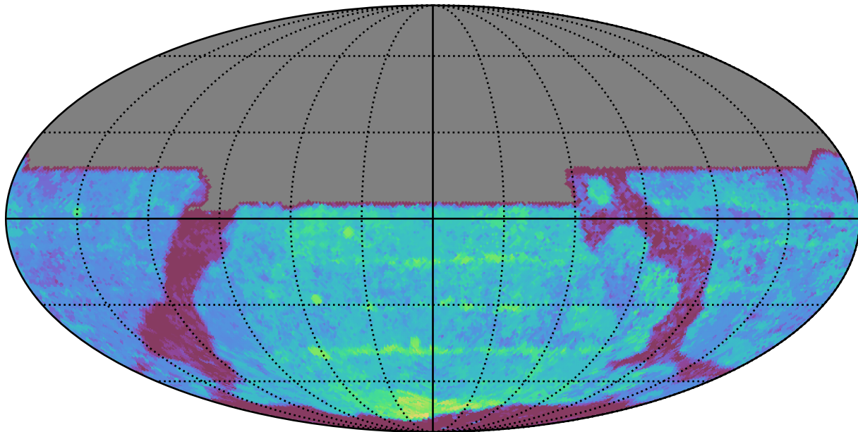
no_magell_roll_v3.4_10yrs All sky y band: Median Season Length
