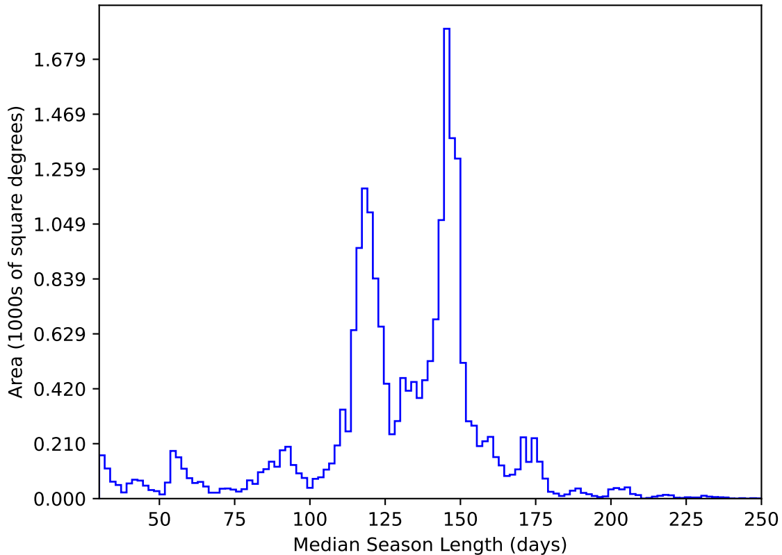
no_magell_roll_v3.4_10yrs All sky y band: Median Season Length
