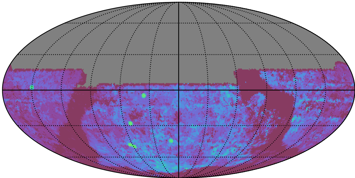
no_magell_roll_v3.4_10yrs All sky u band: Median Season Length
