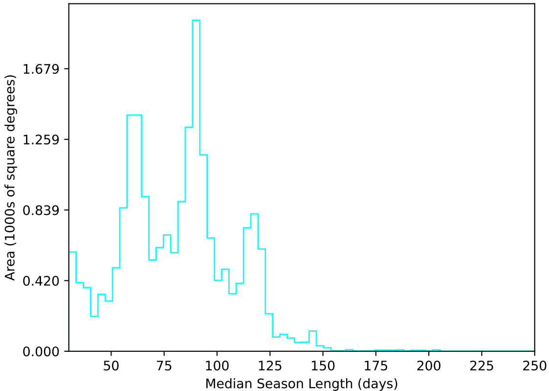
no_magell_roll_v3.4_10yrs All sky u band: Median Season Length
