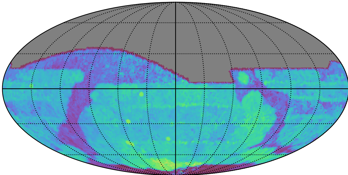
no_magell_roll_v3.4_10yrs All sky i band: Median Season Length
