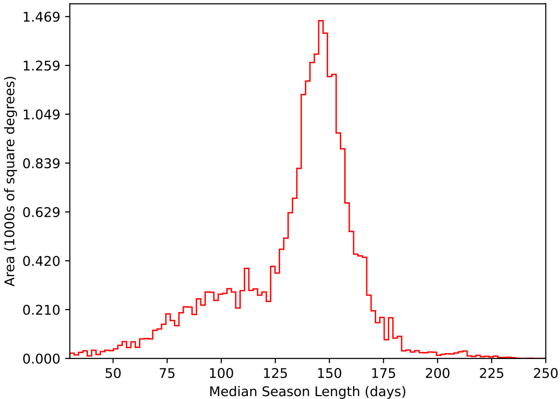
no_magell_roll_v3.4_10yrs All sky i band: Median Season Length
