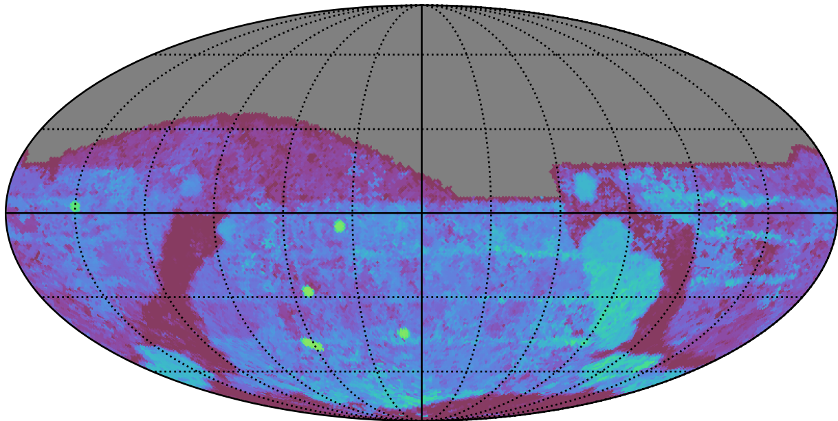
no_magell_roll_v3.4_10yrs All sky g band: Median Season Length
