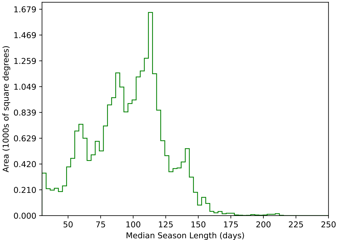
no_magell_roll_v3.4_10yrs All sky g band: Median Season Length
