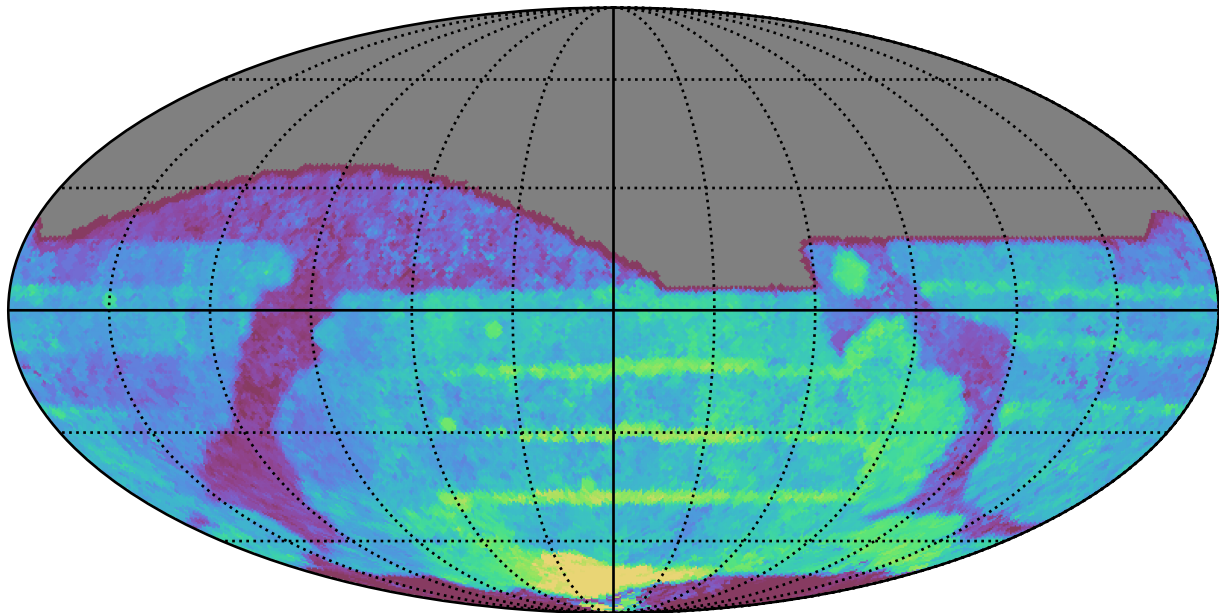
no_magell_roll_v3.4_10yrs All sky all bands: Median Season Length
