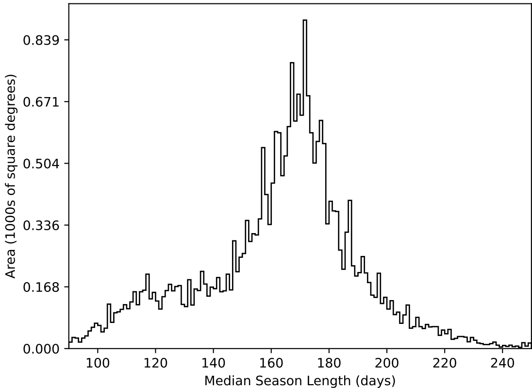
no_magell_roll_v3.4_10yrs All sky all bands: Median Season Length
