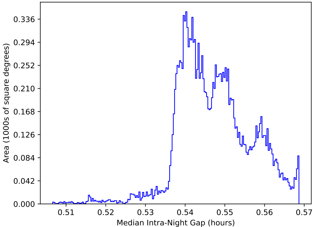
no_magell_roll_v3.4_10yrs WFD: Median Intra-Night Gap
