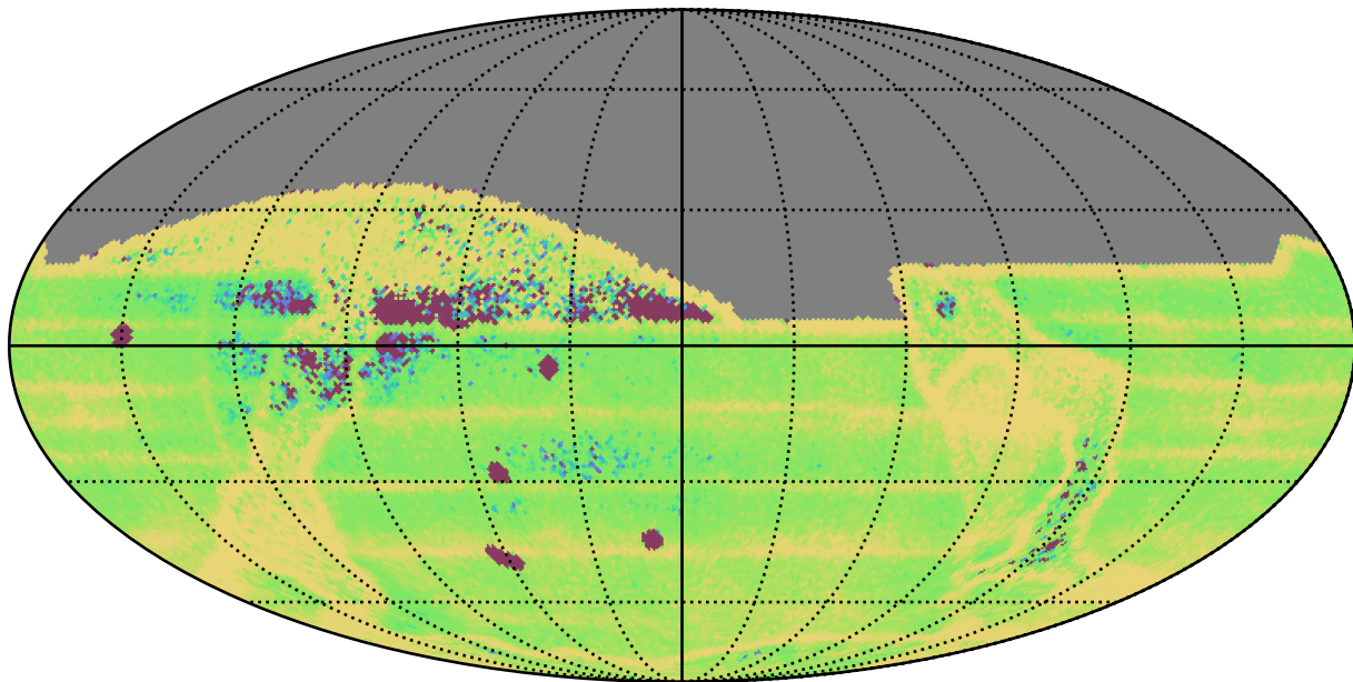
no_magell_roll_v3.4_10yrs All sky: Median Intra-Night Gap
