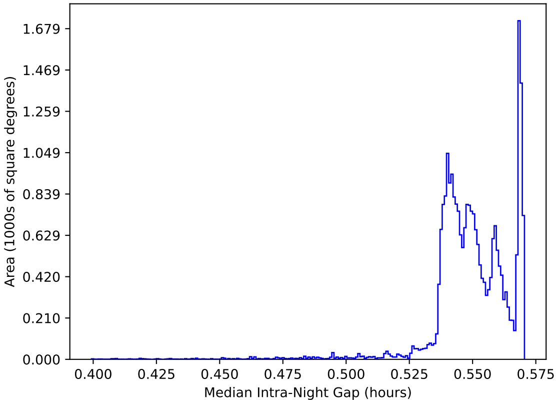
no_magell_roll_v3.4_10yrs All sky: Median Intra-Night Gap
