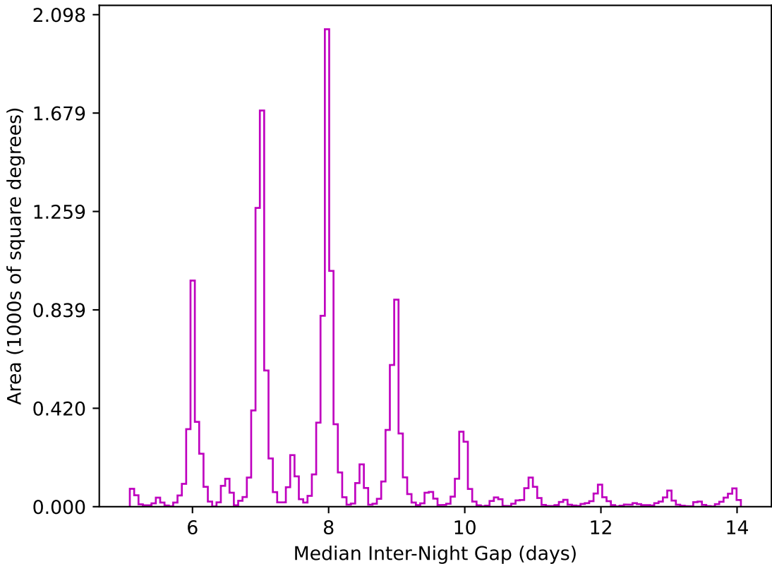
no_magell_roll_v3.4_10yrs WFD z band: Median Inter-Night Gap
