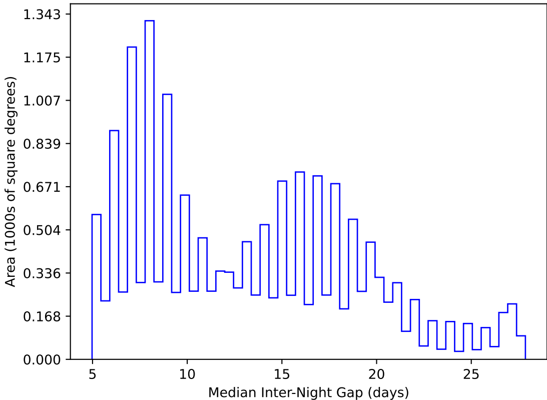
no_magell_roll_v3.4_10yrs WFD y band: Median Inter-Night Gap
