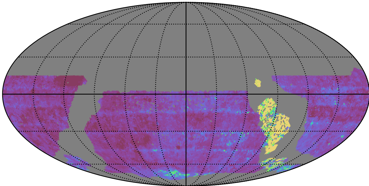
no_magell_roll_v3.4_10yrs WFD u band: Median Inter-Night Gap
