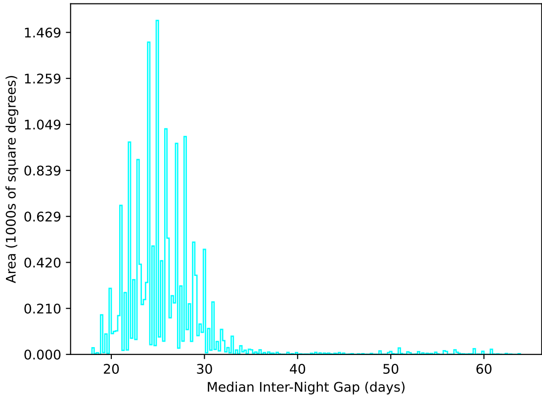
no_magell_roll_v3.4_10yrs WFD u band: Median Inter-Night Gap
