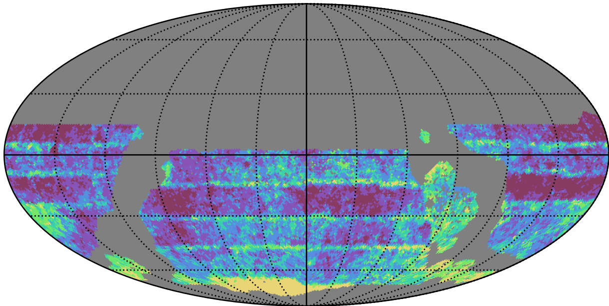
no_magell_roll_v3.4_10yrs WFD r band: Median Inter-Night Gap
