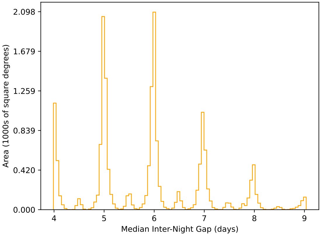
no_magell_roll_v3.4_10yrs WFD r band: Median Inter-Night Gap
