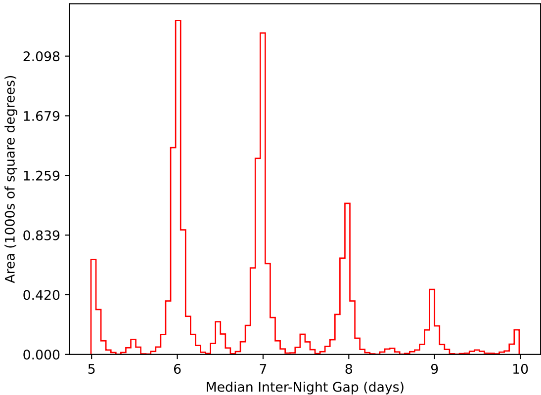
no_magell_roll_v3.4_10yrs WFD i band: Median Inter-Night Gap
