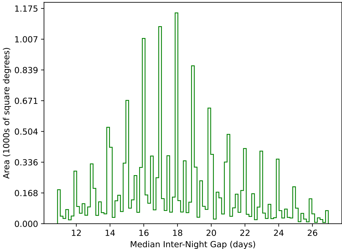
no_magell_roll_v3.4_10yrs WFD g band: Median Inter-Night Gap
