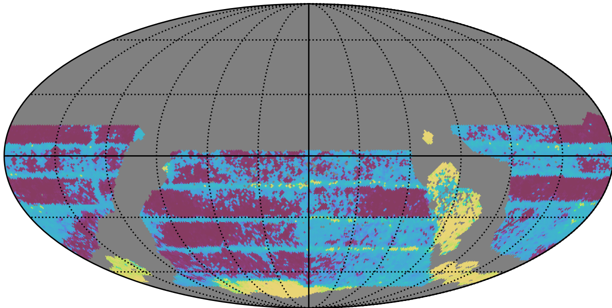
no_magell_roll_v3.4_10yrs WFD all bands: Median Inter-Night Gap
