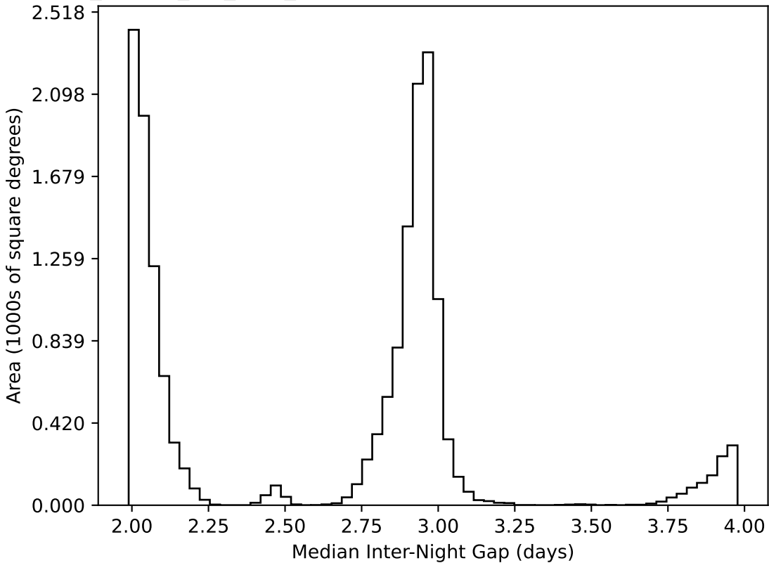
no_magell_roll_v3.4_10yrs WFD all bands: Median Inter-Night Gap
