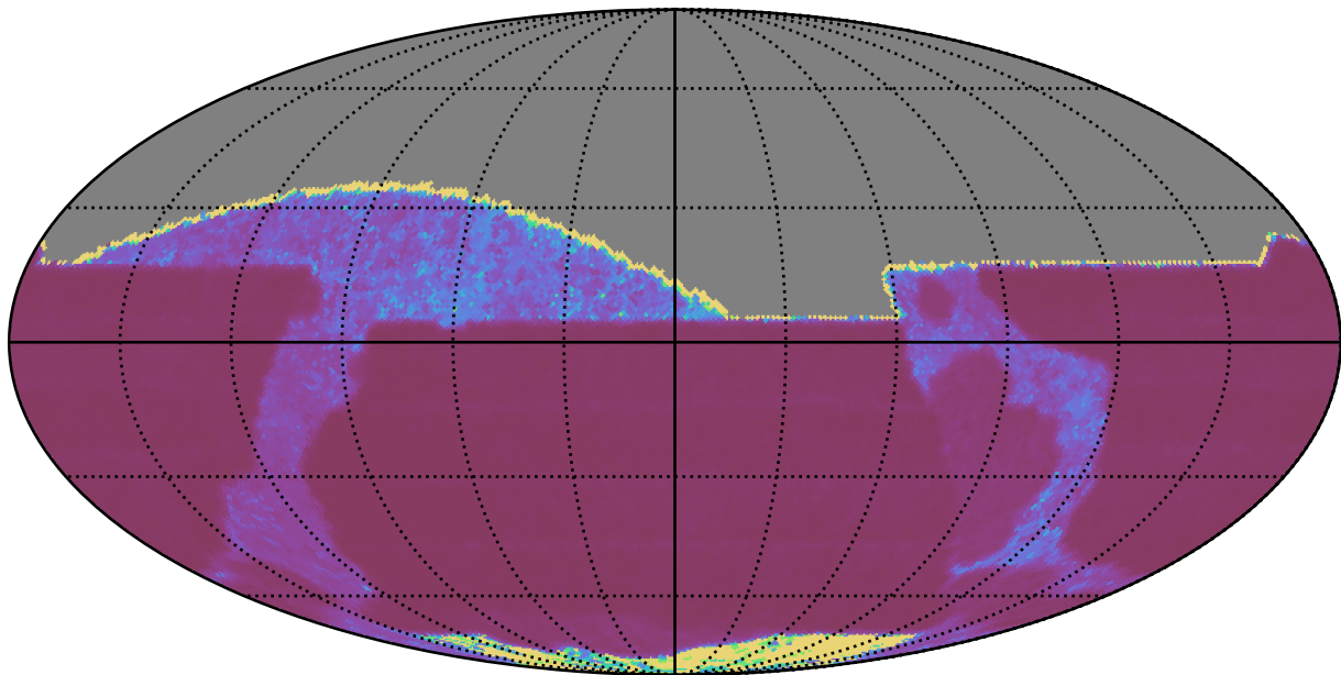
no_magell_roll_v3.4_10yrs All sky z band: Median Inter-Night Gap
