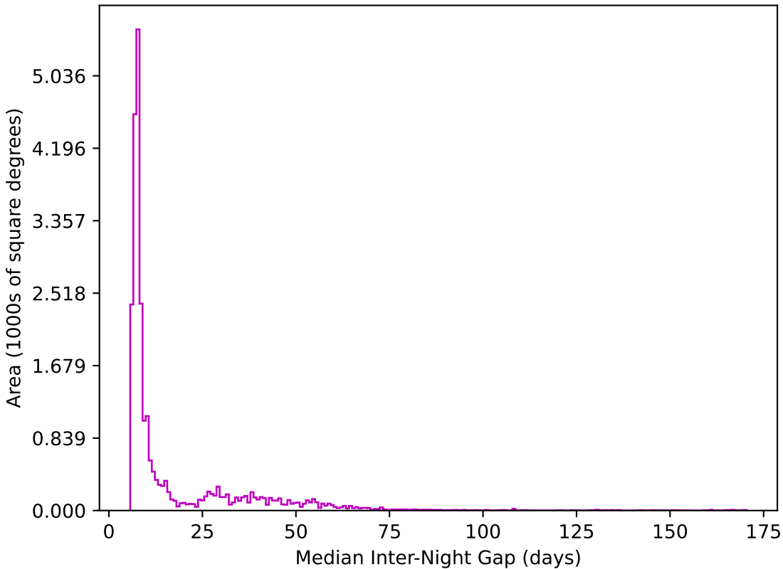
no_magell_roll_v3.4_10yrs All sky z band: Median Inter-Night Gap
