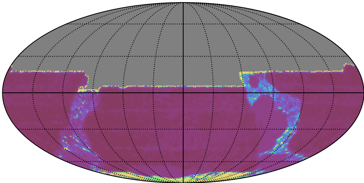
no_magell_roll_v3.4_10yrs All sky y band: Median Inter-Night Gap
