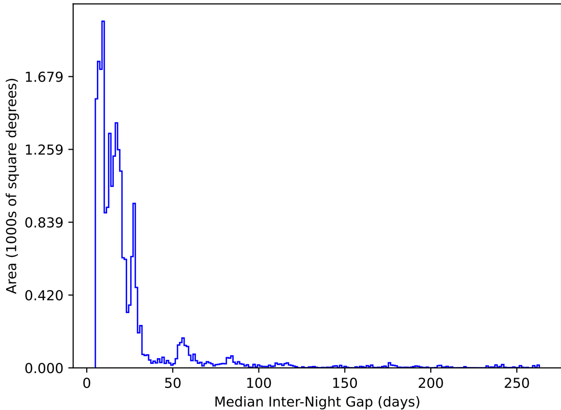
no_magell_roll_v3.4_10yrs All sky y band: Median Inter-Night Gap
