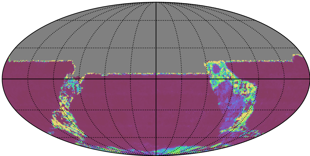
no_magell_roll_v3.4_10yrs All sky u band: Median Inter-Night Gap
