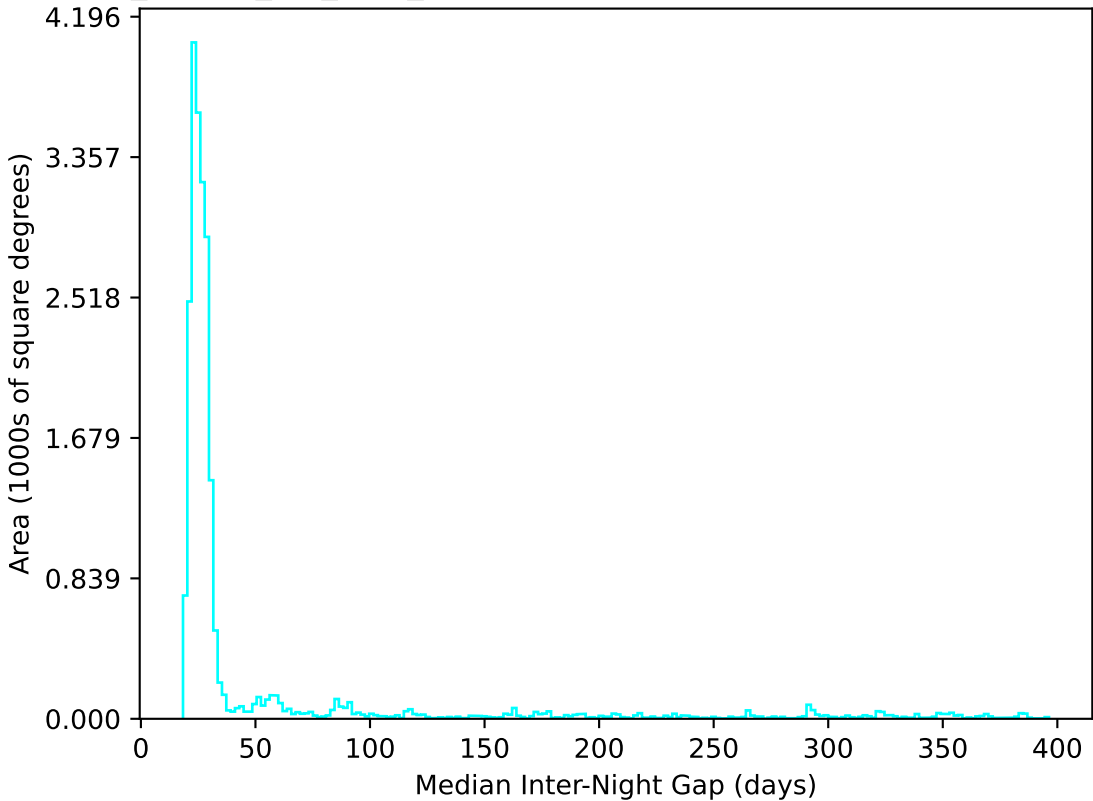
no_magell_roll_v3.4_10yrs All sky u band: Median Inter-Night Gap
