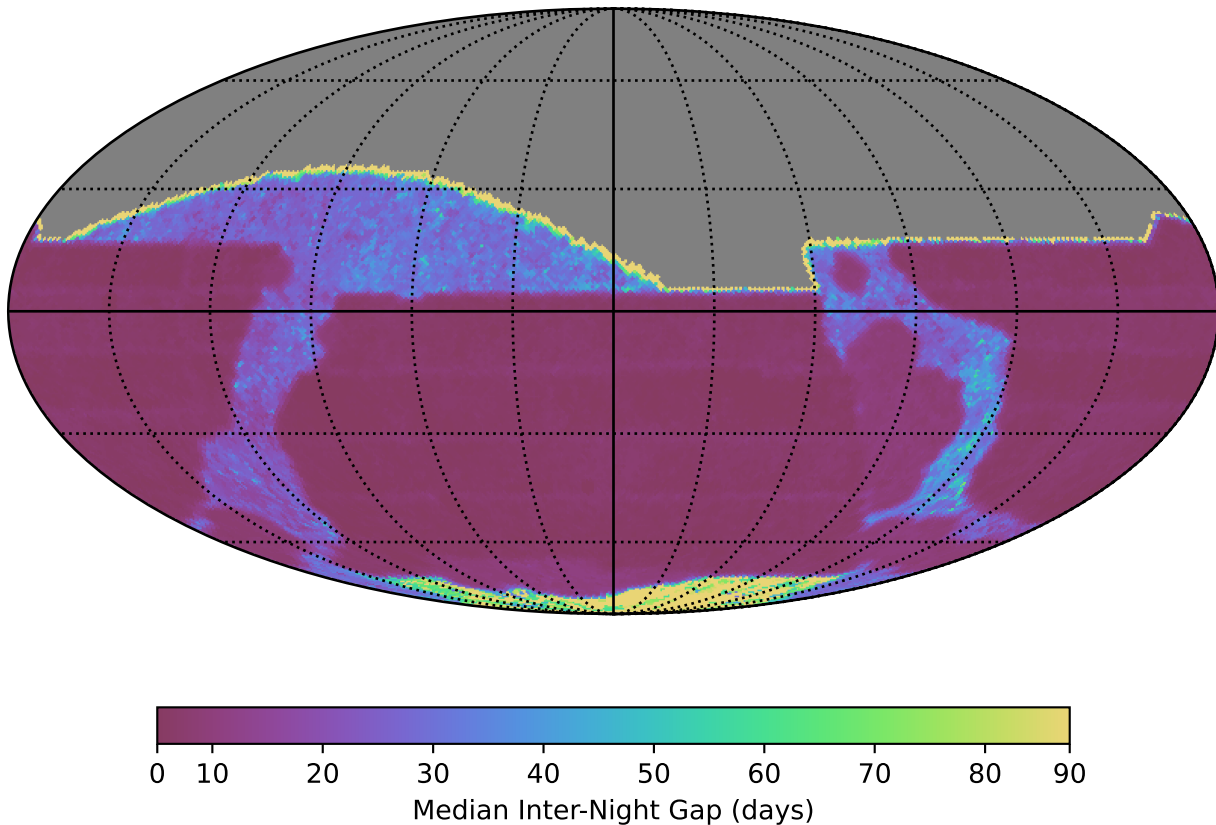
no_magell_roll_v3.4_10yrs All sky i band: Median Inter-Night Gap
