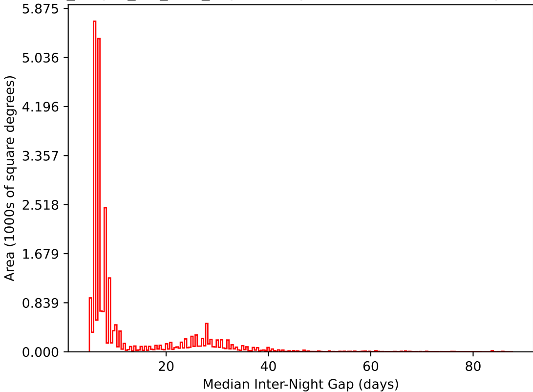
no_magell_roll_v3.4_10yrs All sky i band: Median Inter-Night Gap
