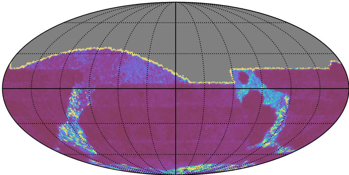
no_magell_roll_v3.4_10yrs All sky g band: Median Inter-Night Gap
