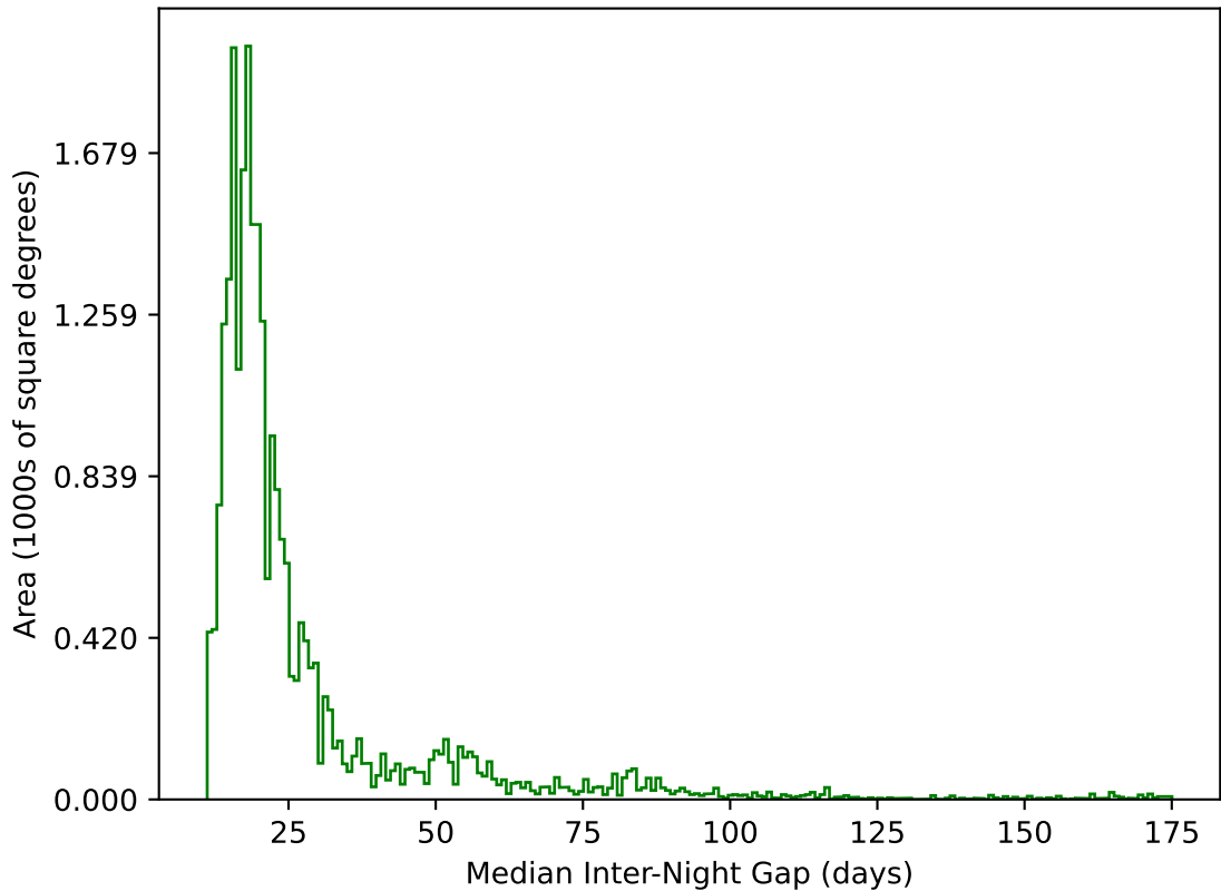
no_magell_roll_v3.4_10yrs All sky g band: Median Inter-Night Gap
