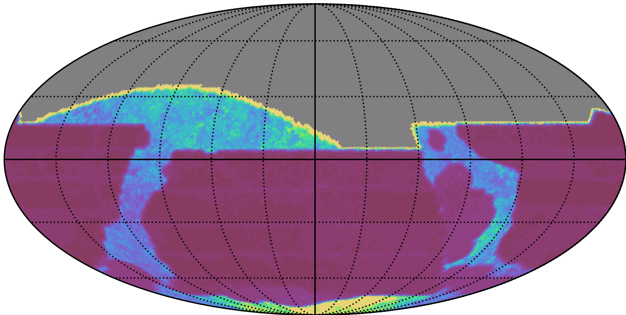
no_magell_roll_v3.4_10yrs All sky all bands: Median Inter-Night Gap
