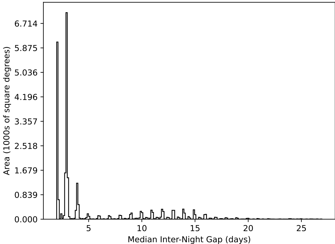
no_magell_roll_v3.4_10yrs All sky all bands: Median Inter-Night Gap
