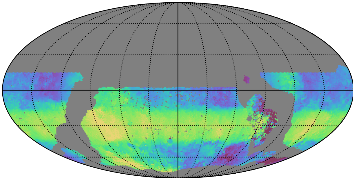
no_magell_roll_v3.4_10yrs WFD u band: Median HA
