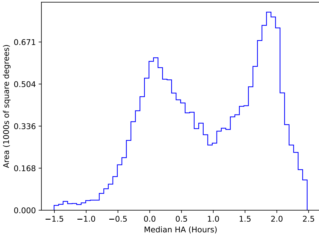
no_magell_roll_v3.4_10yrs WFD u band: Median HA
