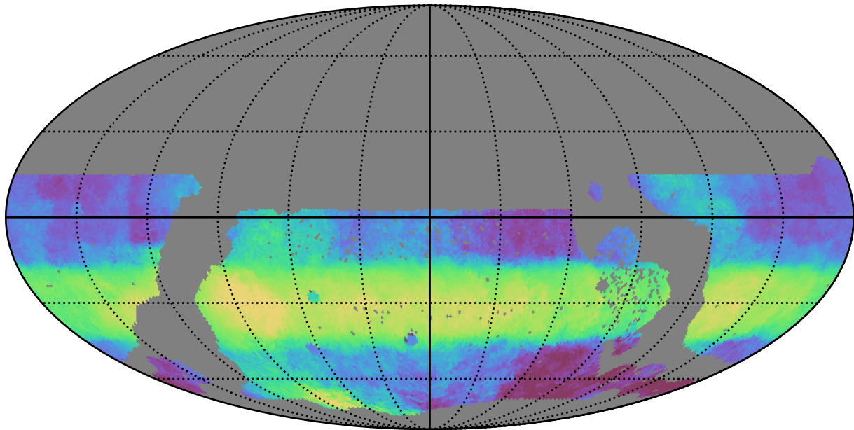
no_magell_roll_v3.4_10yrs WFD r band: Median HA
