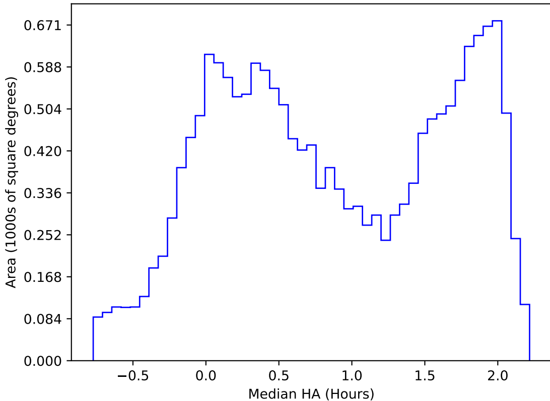
no_magell_roll_v3.4_10yrs WFD r band: Median HA
