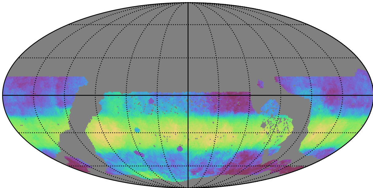
no_magell_roll_v3.4_10yrs WFD i band: Median HA
