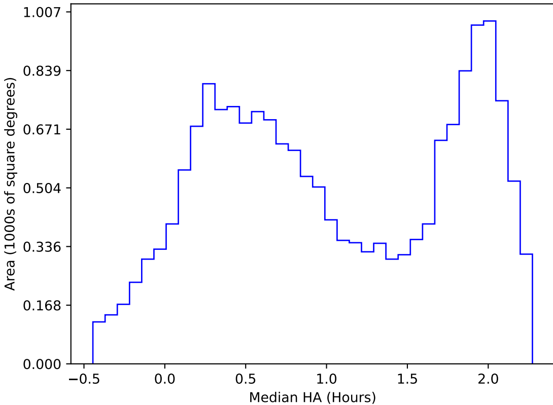
no_magell_roll_v3.4_10yrs WFD i band: Median HA
