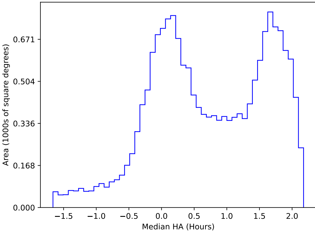
no_magell_roll_v3.4_10yrs WFD g band: Median HA
