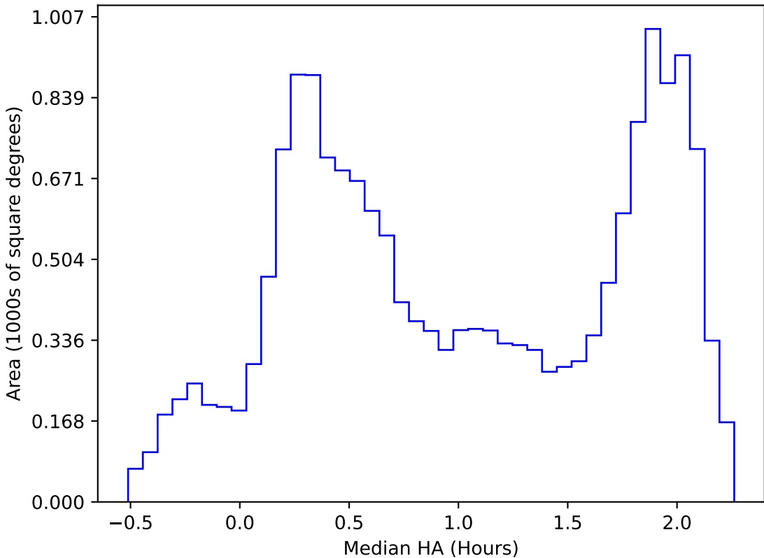
no_magell_roll_v3.4_10yrs WFD all bands: Median HA
