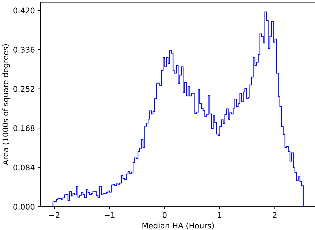
no_magell_roll_v3.4_10yrs All sky u band: Median HA
